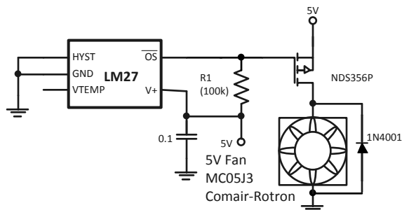
Figure 9. Fan High Side Drive
