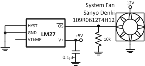
Figure 8. Two Speed Fan Speed Control
