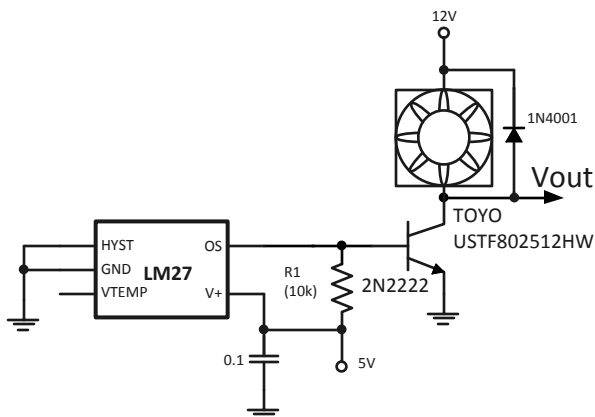
Figure 10. Fan Low Side Drive
