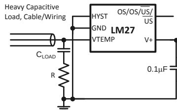
Figure 6. R in series with capacitor
