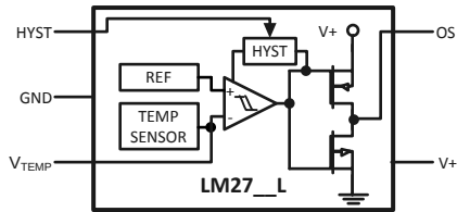
Figure 4. LM27-__L
