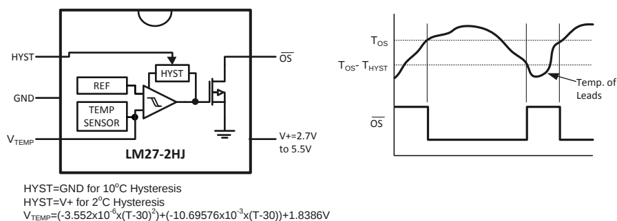
Figure 1. The LM27CIM5-2HJ has a fixed trip point of 140°C For other trip point and output function availability, please see ordering information or contact Texas Instruments
