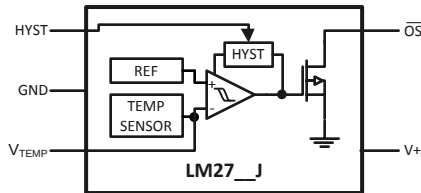
Figure 2. LM27-__J
