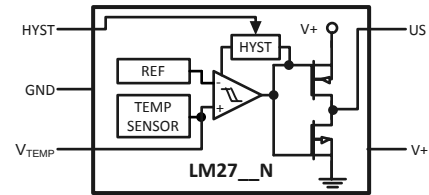
Figure 5. LM27-__N
