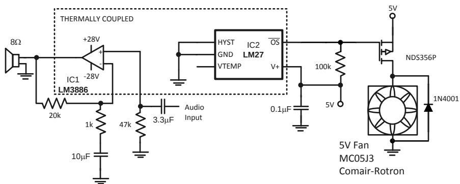
Figure 11. Audio Power Amplifier Thermal Protection
