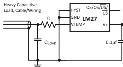
Figure 7. R in series with signal path
