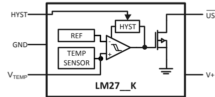
Figure 3. LM27-__K
