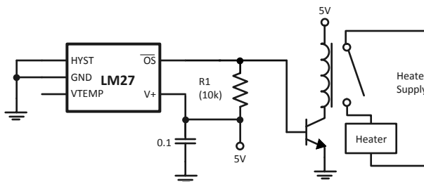
Figure 12. Simple Thermostat
