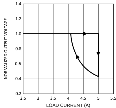
Figure 6. Normalized Output Voltage Versus Load Current
