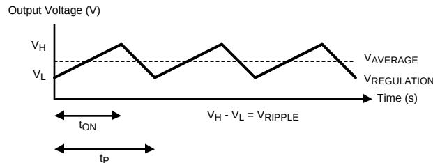
Figure 9. Average Output Voltage and Regulation Point
