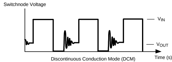
Figure 7. Modes of Operation
