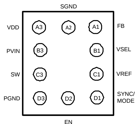
Figure 3. BOTTOM VIEW
