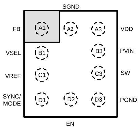
Figure 2. TOP VIEW
