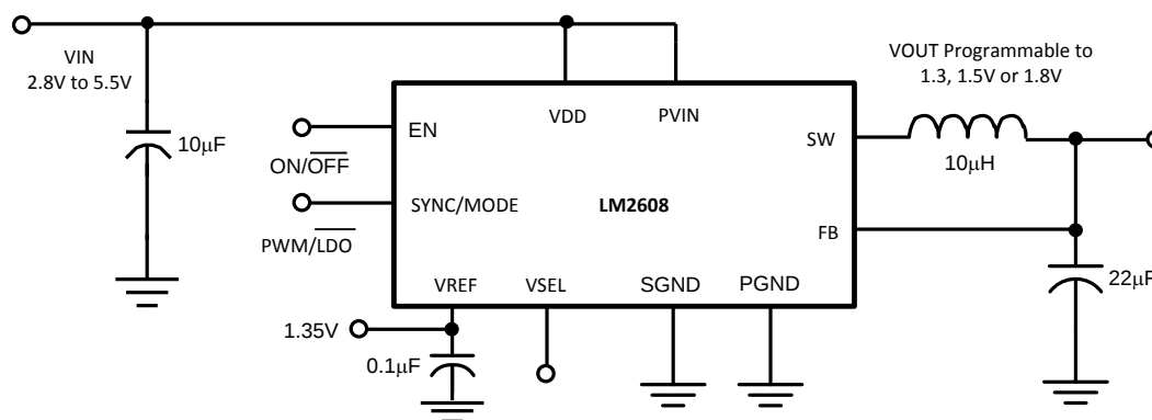
Figure 1. Application Circuit
