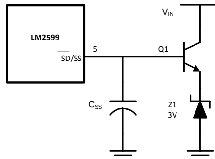
Figure 31. External 3.7V Soft-Start Clamp
