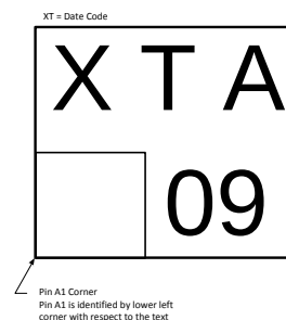
Figure 7. Top View - LM2904ITP micro SMD Marking Orientation
