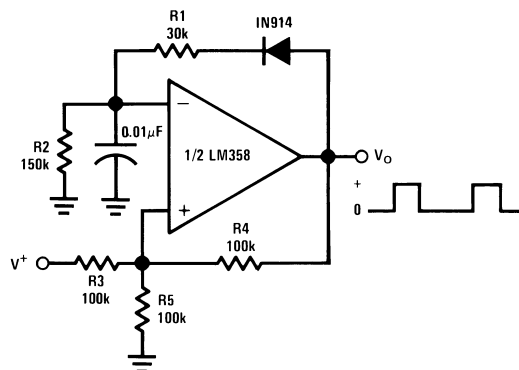
Figure 20. Pulse Generator
