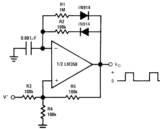
Figure 18. Pulse Generator
