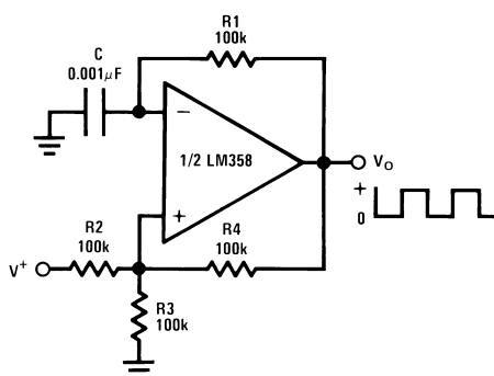
Figure 19. Squarewave Oscillator
