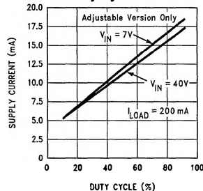
Supply Current vs Duty Cycle
