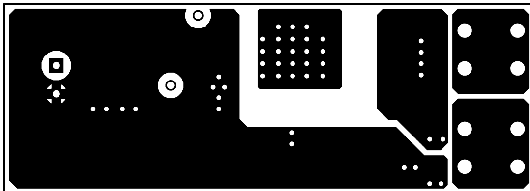
Figure 23. Solder Side
