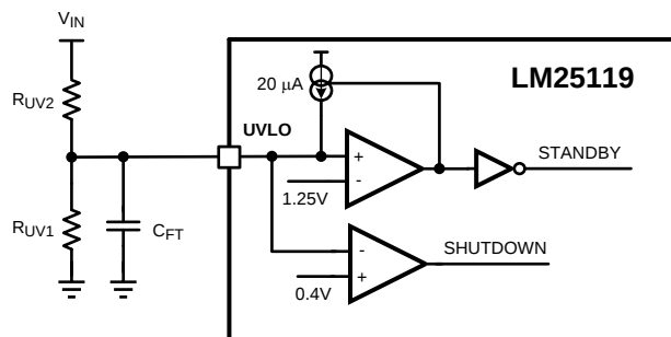
Figure 9. UVLO Configuration
