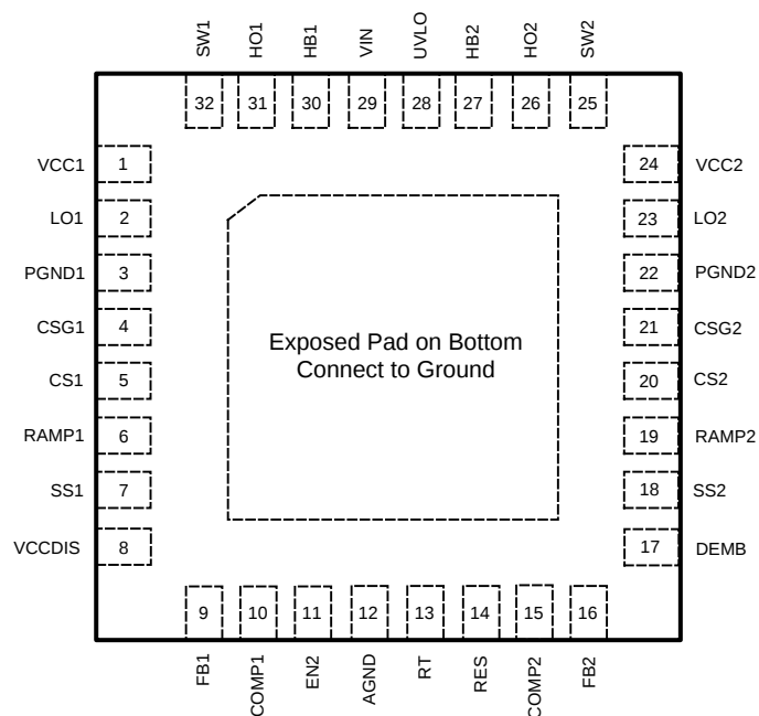
Figure 1. Top View 32-Lead LLP
