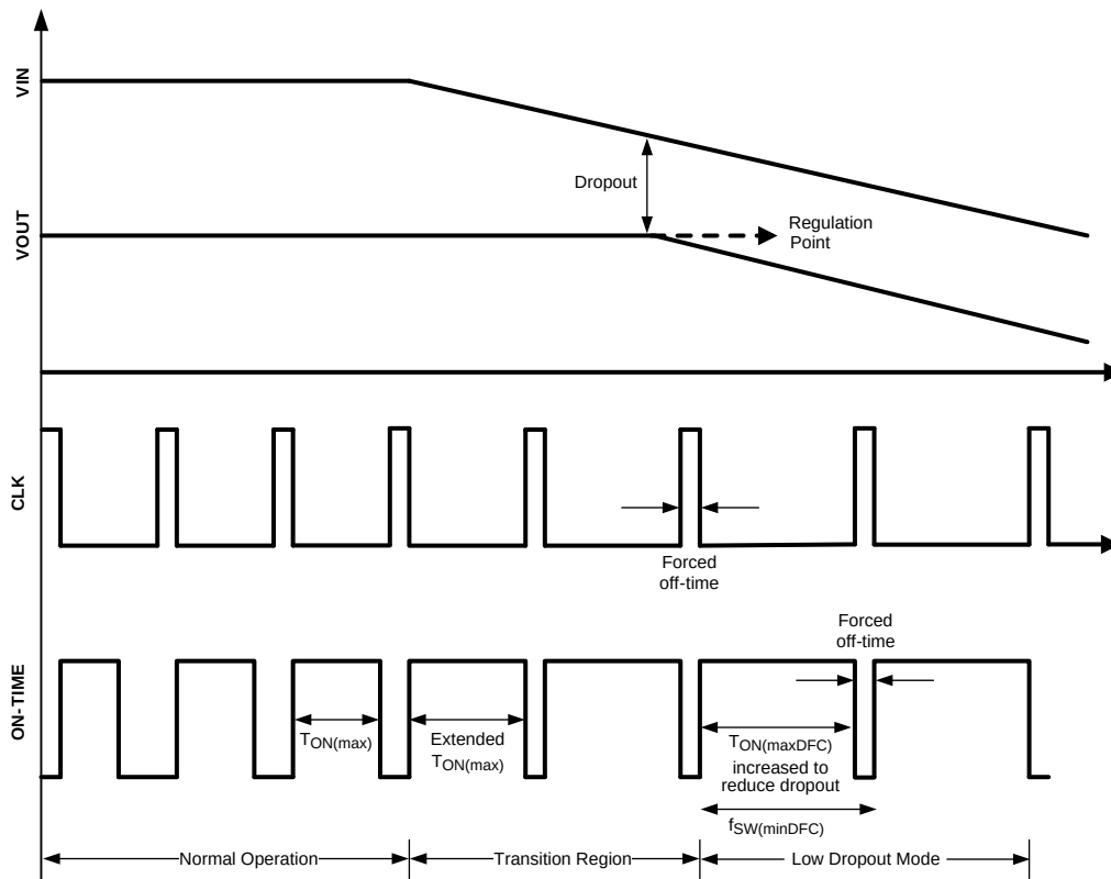
Figure 18. Dropout Voltage Reduction using Dynamic Frequency Control
