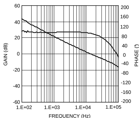
Figure 27. Overall Loop Gain and Phase
