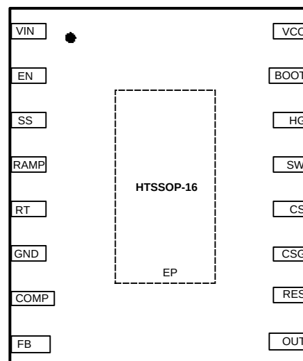
Figure 2. Top View (Restart version) LM25088-2
