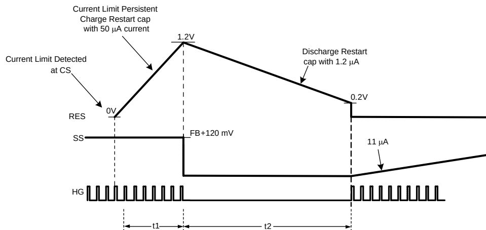
Figure 22. Current Limit Restart Timing Diagram
