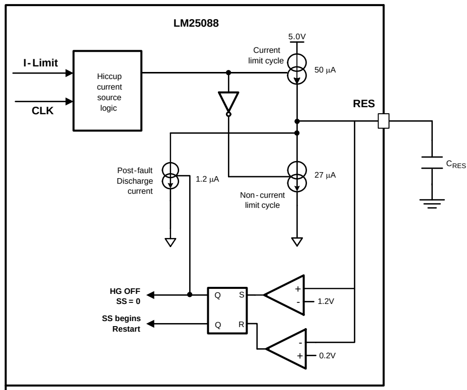
Figure 21. Current Limit Restart Circuit
