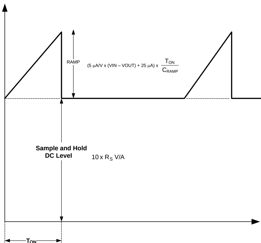
Figure 17. Composition of Current Sense Signal
