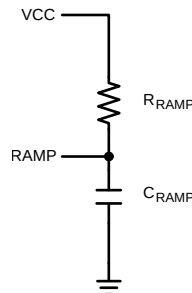
Figure 24. Additional Slope Compensation for V_{\text{OUT}} > 5\text{V}
