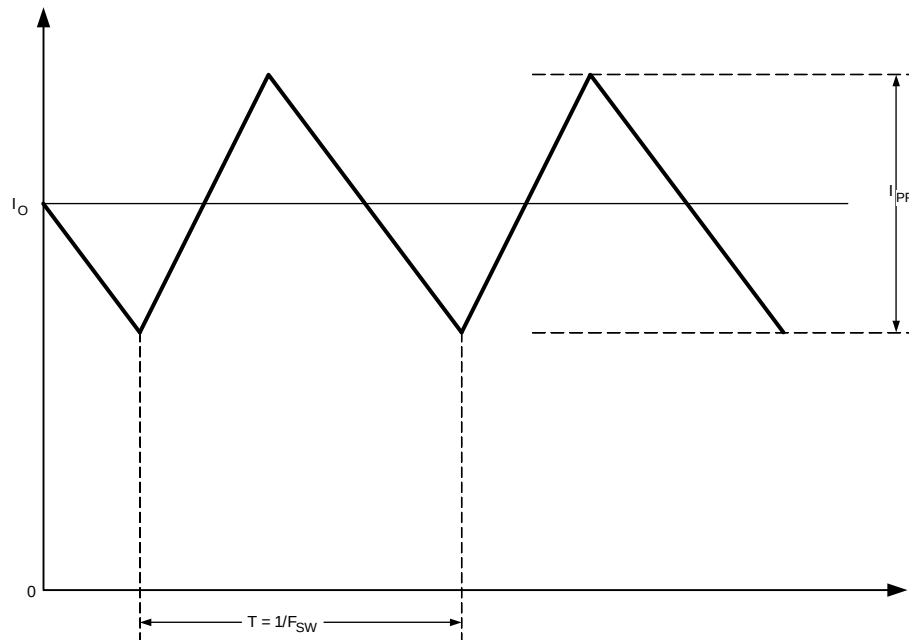
Figure 23. Inductor Current
