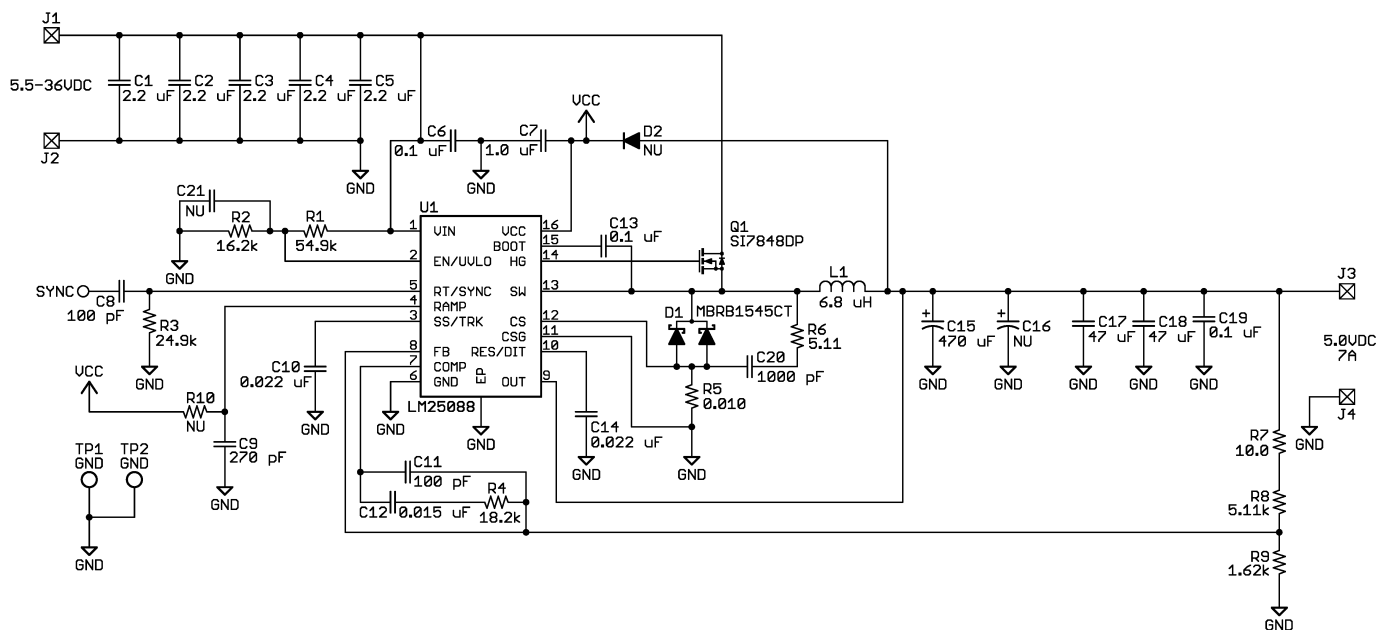
Figure 29. LM25088-2 Application Schematic
