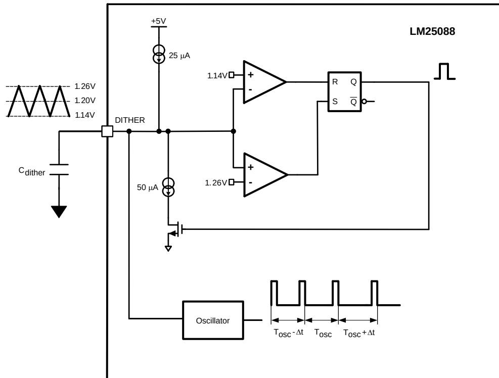
Figure 19. Frequency Dithering Scheme
