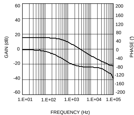
Figure 25. Modular Gain Phase
