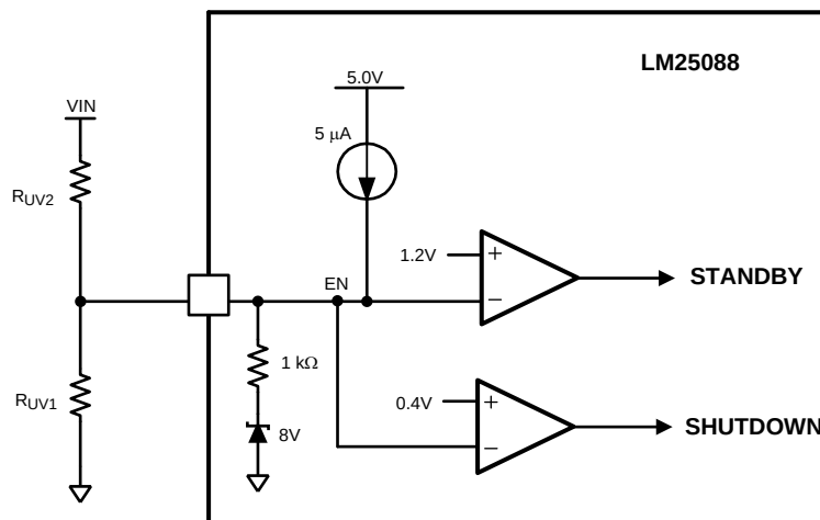
Figure 16. Basic Enable Configuration
