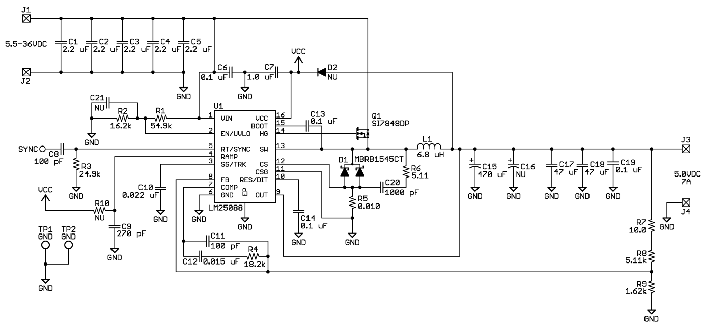
Figure 28. LM25088-1 Application Schematic
