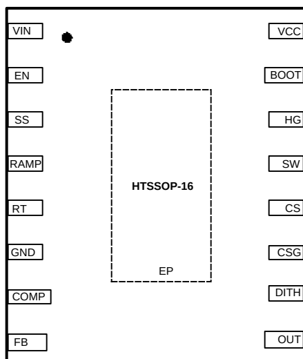
Figure 1. Top View (Dither version) LM25088-1
