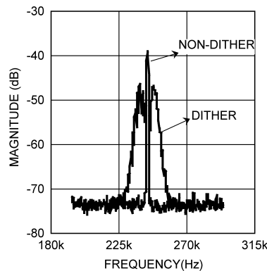
Figure 20. Conducted Emissions Measured at the Input of a LM25088 Based Buck Converter
