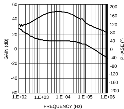
Figure 26. Error Amplifier Gain and Phase
