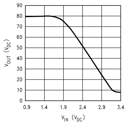
FIGURE 5. CRT Driver V_O vs V_{IN}
