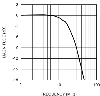
Figure 6. Bandwidth
