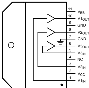
Figure 1. Top View Available only with lead free plating
