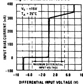
Input Characteristics
