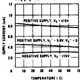
Supply Currents
