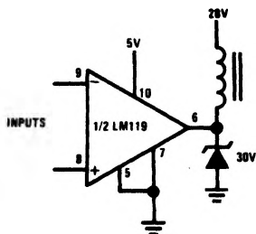
Relay Driver
