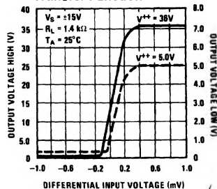
Transfer Function
