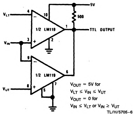
Window Detector
