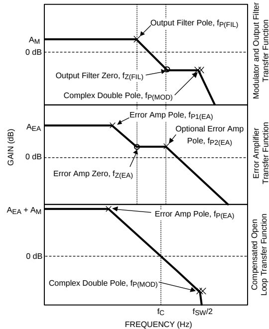
Figure 4. LM20343 Loop Compensation
