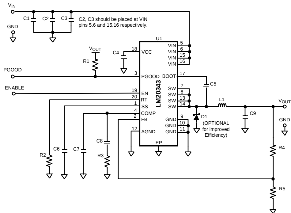
Figure 15. Typical Application Schematic
