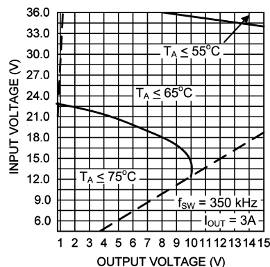
Figure 9. Safe Thermal Operating Areas ( I_{OUT} = 3A , f_{SW} = 350kHz )
