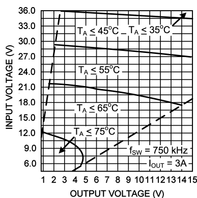
Figure 11. Safe Thermal Operating Areas ( I_{OUT} = 3A , f_{SW} = 750 kHz)
