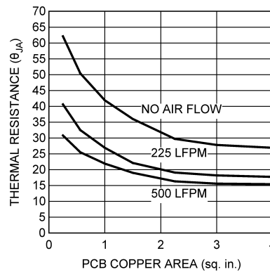
Figure 13. Thermal Resistance vs PCB Area
