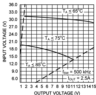
Figure 12. Safe Thermal Operating Areas ( I_{OUT} = 2.5A , f_{SW} = 500 kHz)
