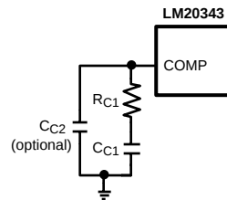
Figure 5. Compensation Network for LM20343
