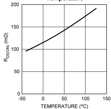
Low-Side FET Resistance vs. Temperature
