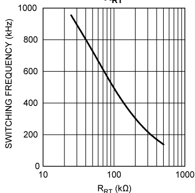
Oscillator Frequency vs. R_{RT}
