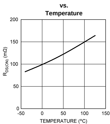
Low-Side FET Resistance
