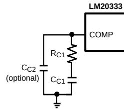
Figure 5. Compensation Network for LM20333
