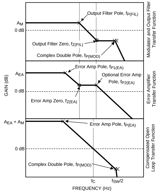
Figure 4. LM20333 Loop Compensation
