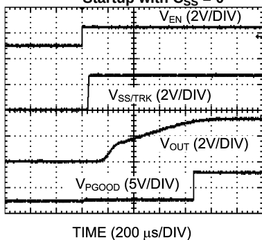
Startup with C_{SS} = 0
