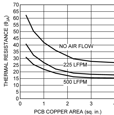
Figure 13. Thermal Resistance vs PCB Area (4 Layer Board)
