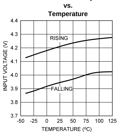
UVLO Threshold and Hysteresis
