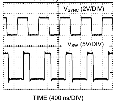
Clock Synchronization
