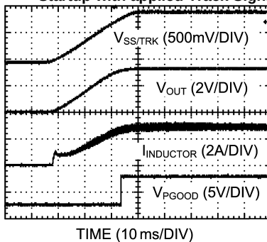
Startup with applied Track Signal
