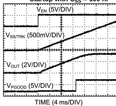
Startup with C_{SS} = 100 nF
