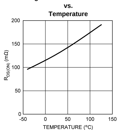
High-Side FET Resistance
