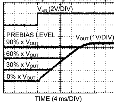
Startup with prebiased output
