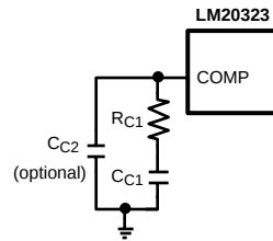
Figure 5. Compensation Network for LM20323
