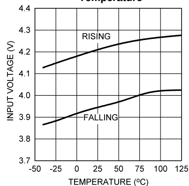
UVLO Threshold and Hysteresis
