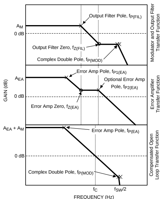
Figure 4. LM20323 Loop Compensation
