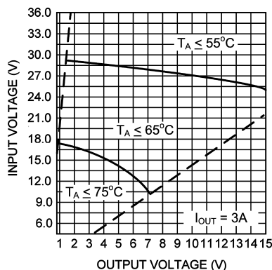
Figure 9. Safe Thermal Operating Areas ( I_{OUT} = 3A )
