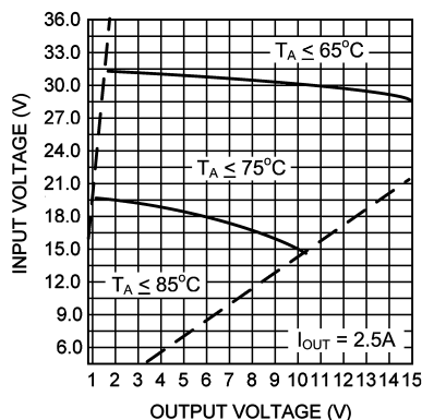
Figure 10. Safe Thermal Operating Areas ( I_{OUT} = 2.5A )
