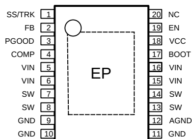
Figure 1. Top View eTSSOP-20 Package
