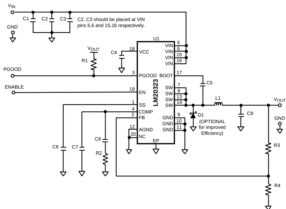
Figure 13. Typical Application Schematic
