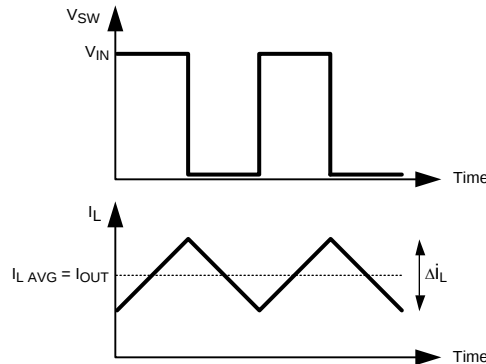
Figure 3. Switch and Inductor Current Waveforms
