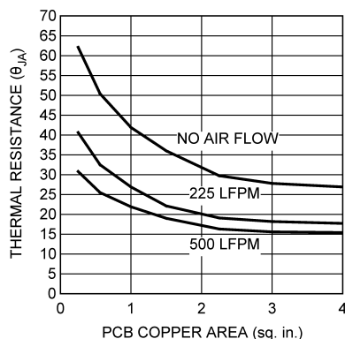
Figure 11. Thermal Resistance vs PCB Area (4 Layer Board)
