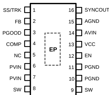
Figure 1. Top View TSSOP-16 Package
