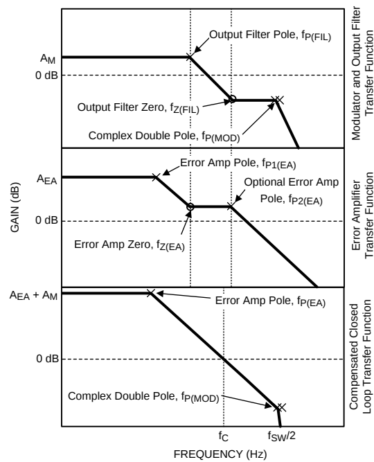
Figure 27. LM20123 Loop Compensation
