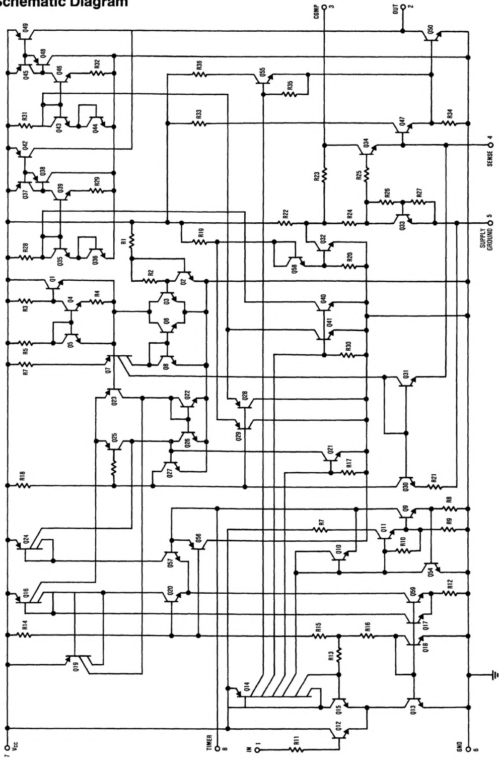
FIGURE 2. LM1949 Circuit
