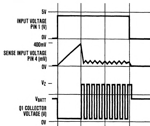
FIGURE 6. Switching Waveforms
