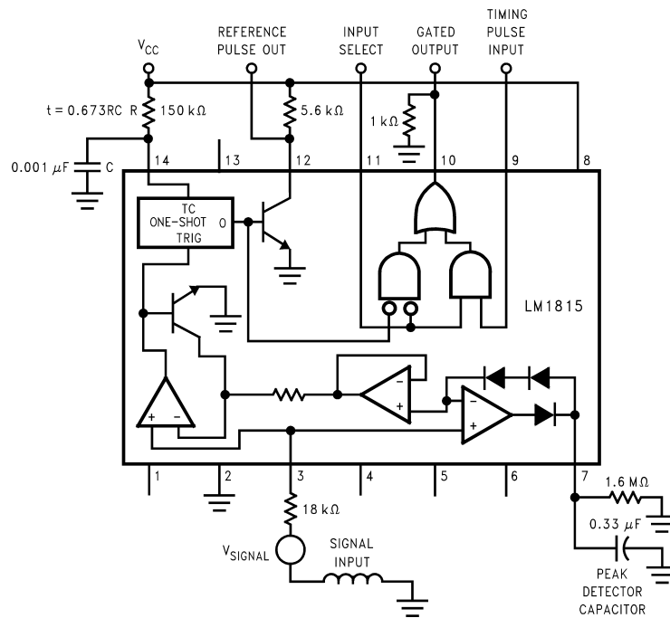
Figure 2. LM1815 Adaptive Sense Amplifier
