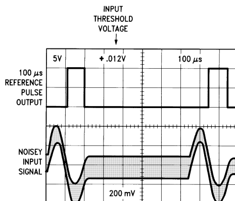
Figure 3. LM1815 Oscilloscopes
