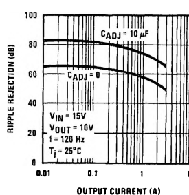
Ripple Rejection
