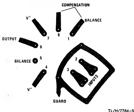
FIGURE 1. Printed Circuit Layout for Input Guarding with TO-5 Package
