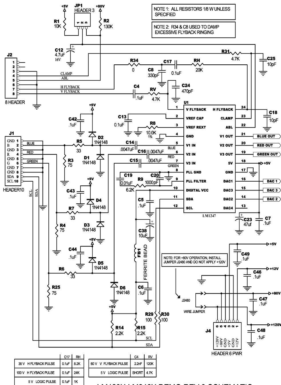
LM123X-LM246X DEMO REV 3 SCHEMATIC
