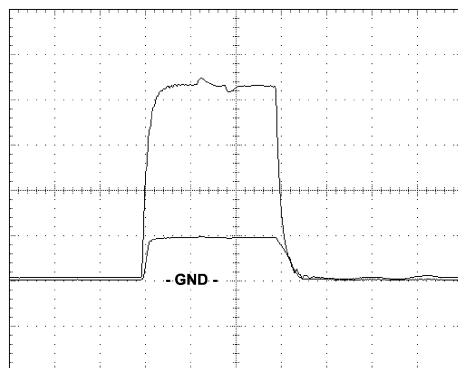
Figure 2. Logic Horizontal Blanking
