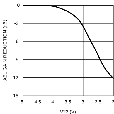
Figure 8. ABL Gain Reduction Curve
