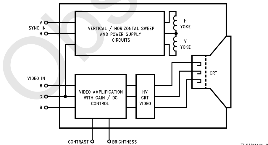
FIGURE 4. Typical RGB Color Monitor Block Diagram
