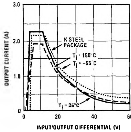
Current Limit
