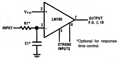
Adjustable Threshold Line Receiver
