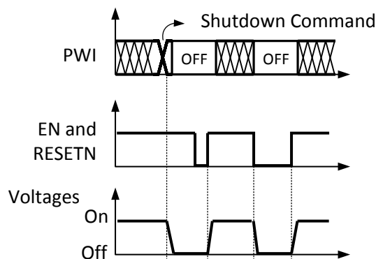
Figure 27. Shutdown And Enable Methods
