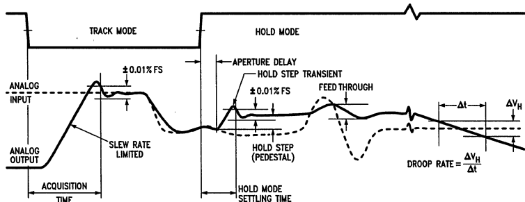
FIGURE 1. Timing Diagram
