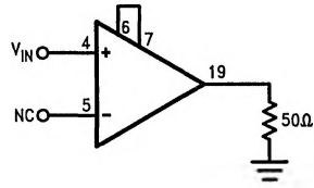
FIGURE 1. Unity Gain Buffer
