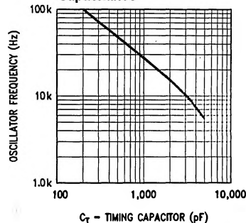
Frequency vs Timing Capacitance
