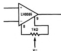
FIGURE 5. Offset Adjustment
