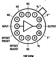
LH0033G Metal Can Package
