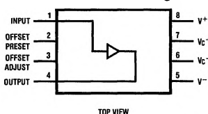
LH0033J Dual-In-Line Package
