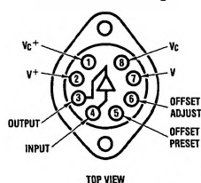
LH0063K Metal Can Package
