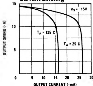
Current Limiting
