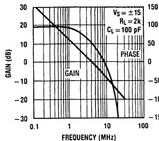
Bode Plot
