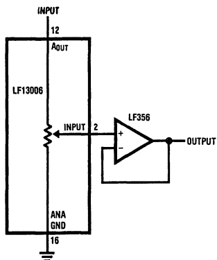
Attenuator (0 dB to -42 dB in 6 dB steps)
