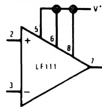
Increasing Input Stage Current*
