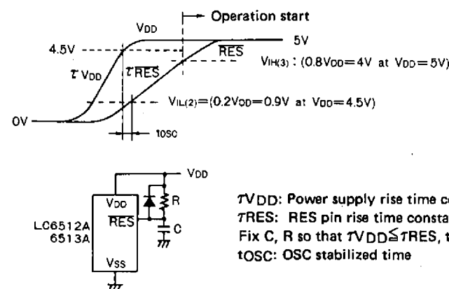
Fig. 5 Initial reset timing
