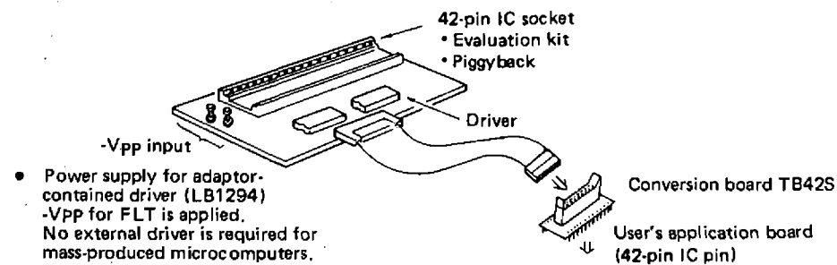
Fig. 1-3 Adaptor (EVA-97-12D/13D) for LC6512A, 6513A
