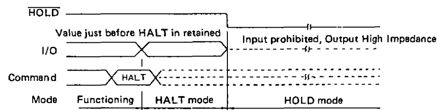
Fig. 4-2 Mode change from HALT mode to HOLD mode
