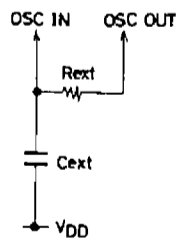
Fig. 11 Recommended CR oscillation circuit
