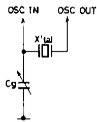
Fig. 7 Recommended crystal oscillation circuit
