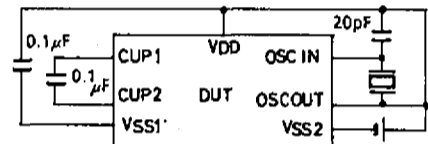
Fig. 5 Current dissipation, output voltage test circuit
