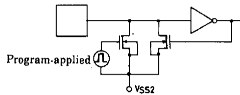
Fig. 4 Input configuration of S1-4, M1-4
