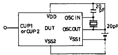
Fig. 3 Oscillation start voltage, oscillation start time, frequency stability, oscillation hold voltage test circuit
