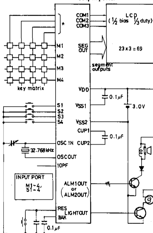
Crystal OSC (Power supply : Li battery version)
