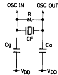
Fig. 12 Recommended ceramic resonator oscillation circuit
