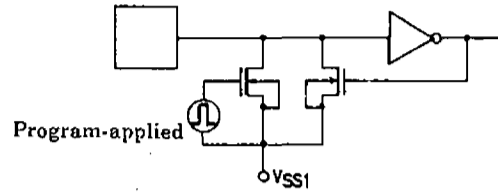
Fig. 1 Input configuration of S1-4, M1-4
