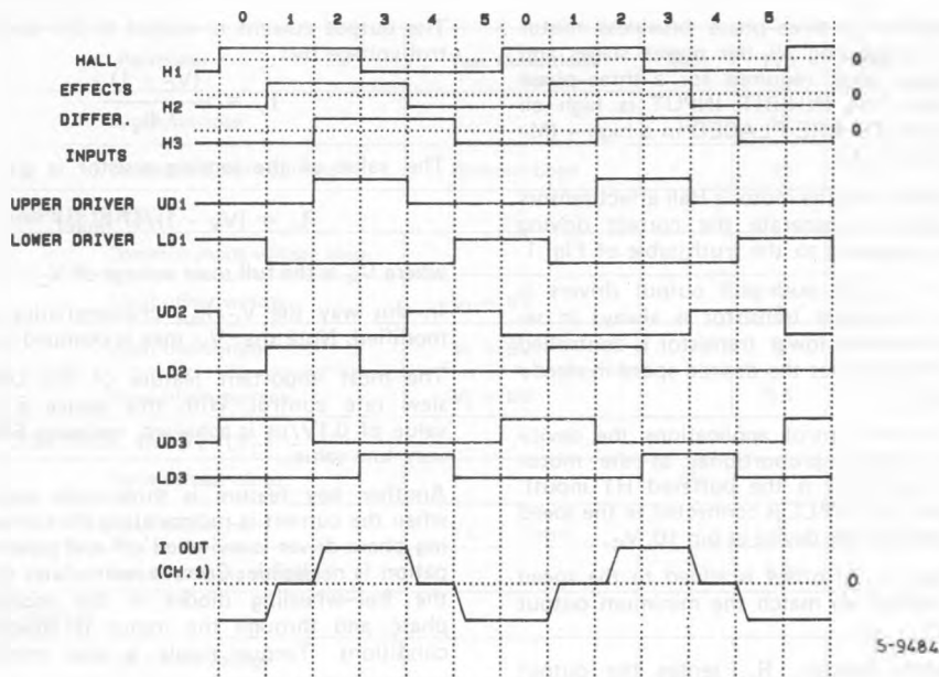
Fig. 2 - Timing diagram
