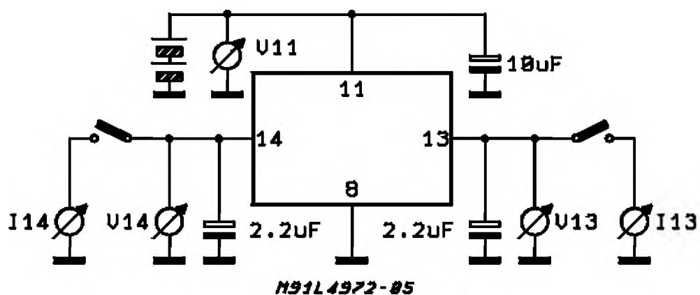
Figure 7 : DC Test Circuits.
