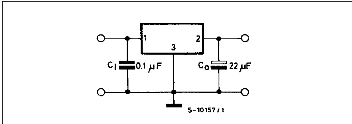
Figure 1 : DC Parameters.
