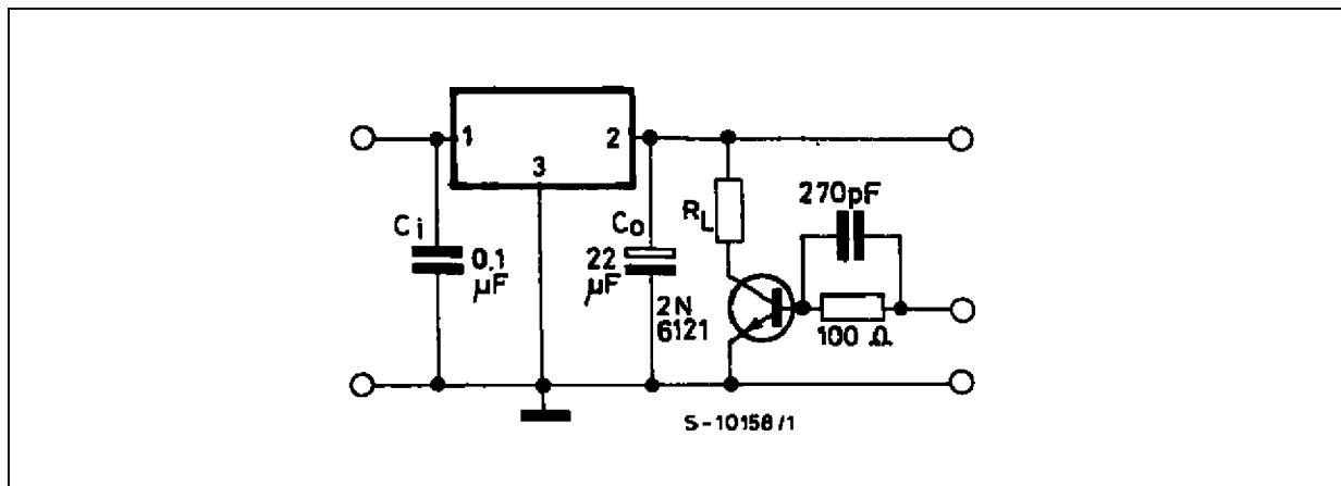
Figure 2 : Load Regulation.
