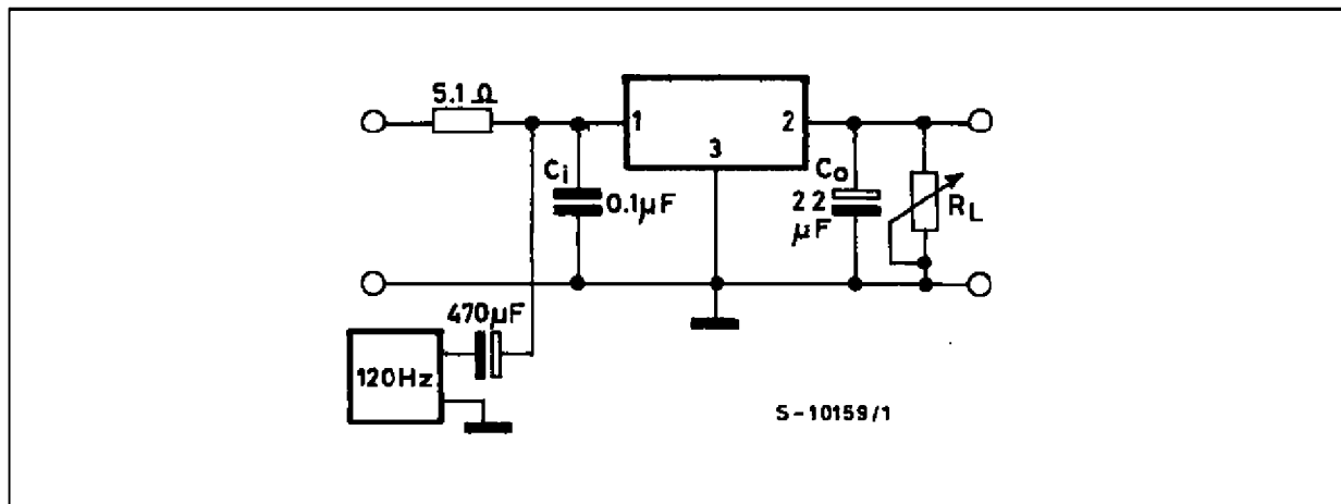
Figure 3 : Ripple Rejection.
