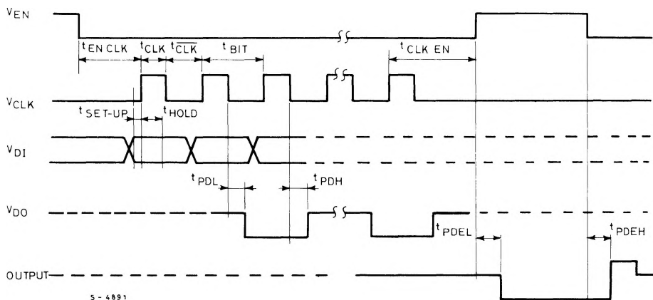
Fig. 1 – Timing diagram
