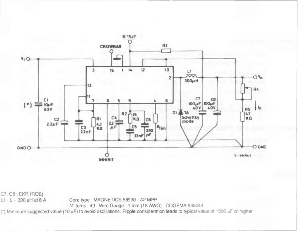
Figure 4 : Dynamic Test Circuit.
