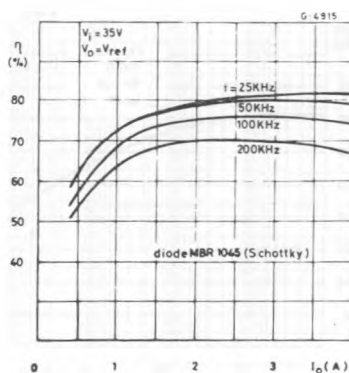
Figure 28 : Efficiency vs. Output Current.
