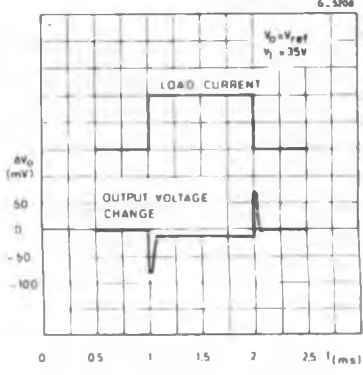
Figure 18 : Load Transient Response (see fig. 4).
