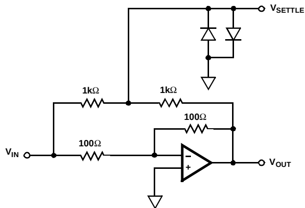
FIGURE 3. SETTLING TIME SCHEMATIC
