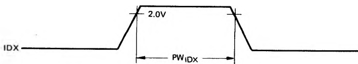
Figure 3 IDX Waveform
