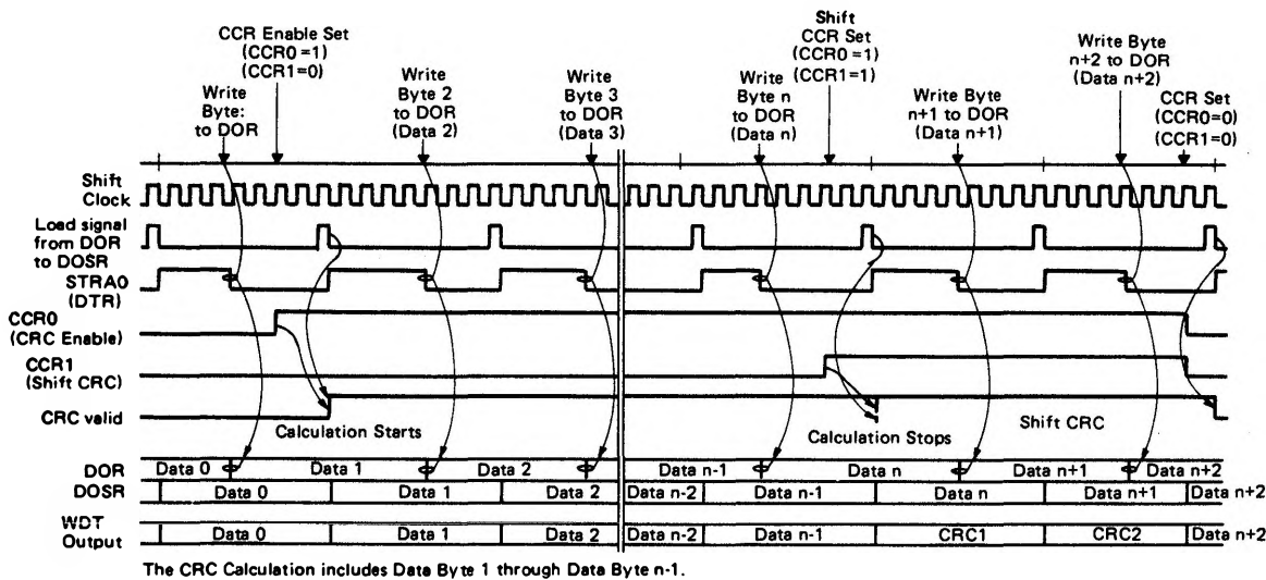
Figure 33 CCR Control Register Timing for an FFW Command (WRITE)
