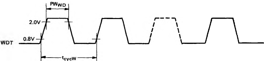
Figure 7 WDT Waveform
