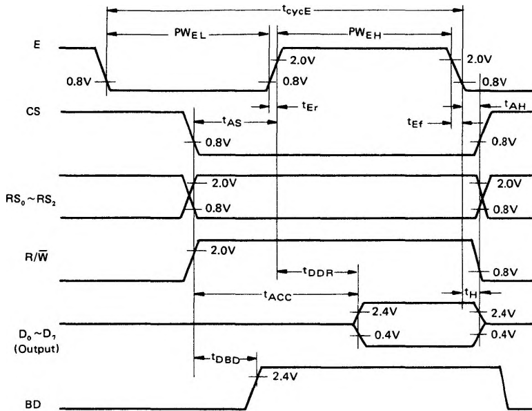
Figure 8 Read Timing
