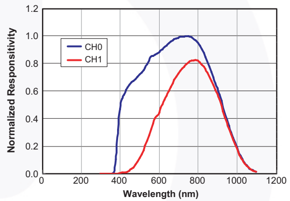
Fig. 4 Spectral Response
