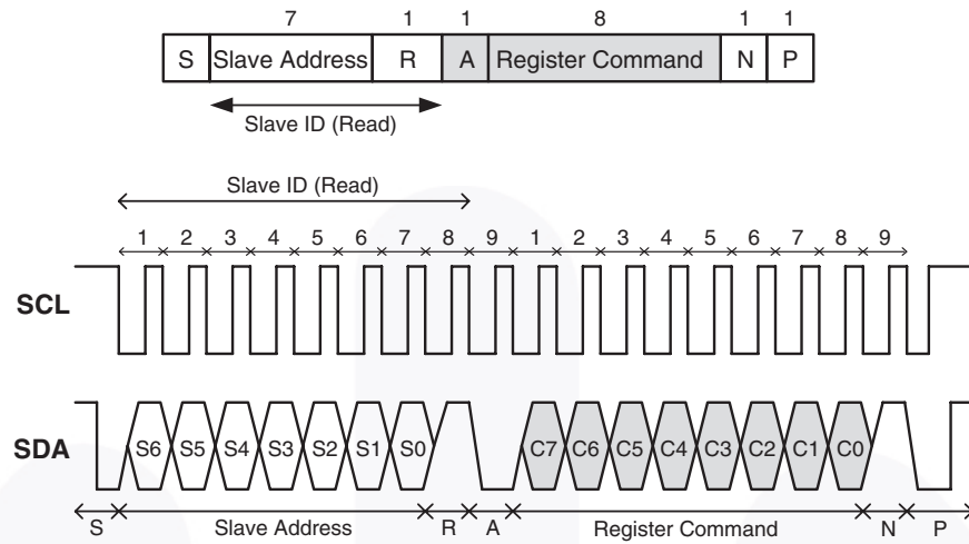
Figure 8. I 2 C Read Protocol
