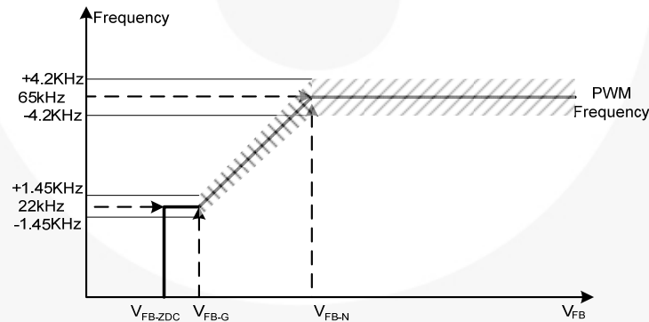
Figure 10. PWM Frequency
