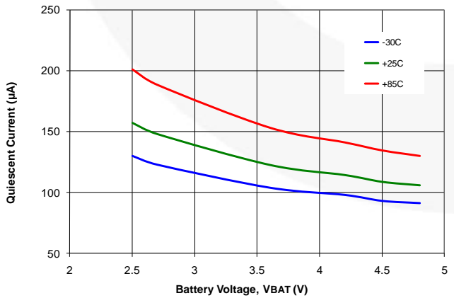
Figure 23. Quiescent Current
