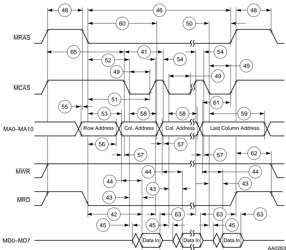
Figure 2-9 DRAM Page Mode Read Cycle
