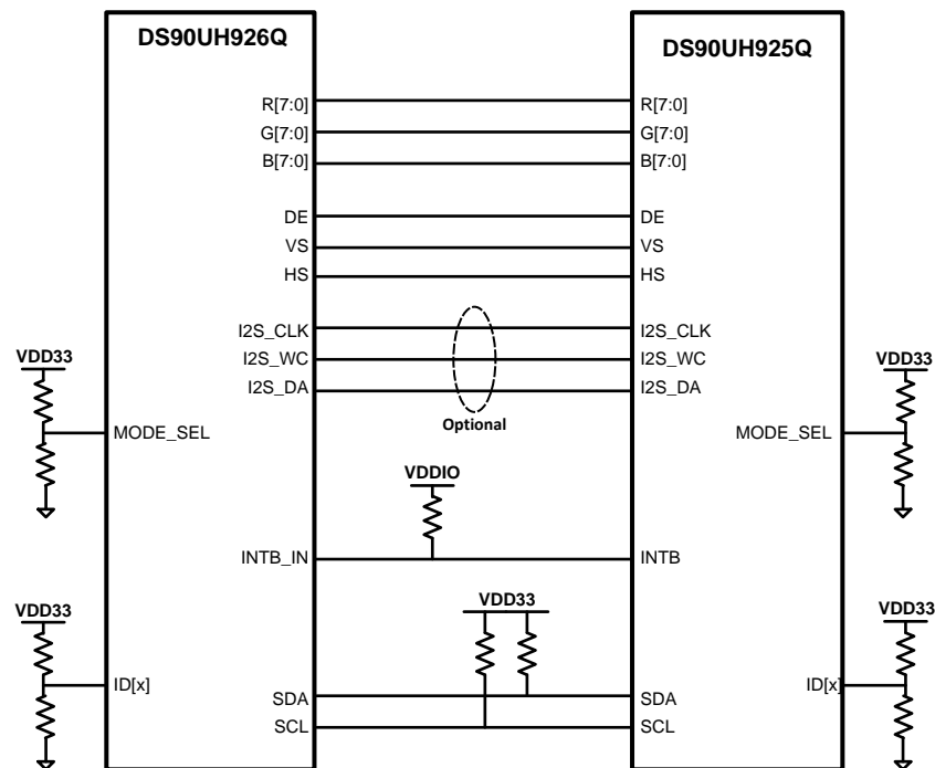
Figure 15. HDCP Repeater Connection Diagram
