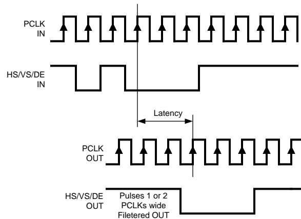
Figure 11. Video Control Signal Filter Waveform
