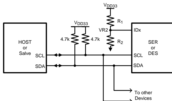
Figure 18. Serial Control Bus Connection
