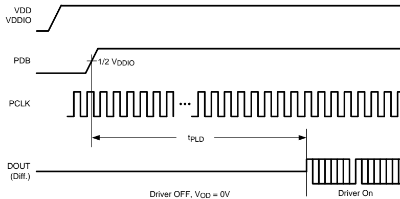
Figure 7. Serializer Lock Time
