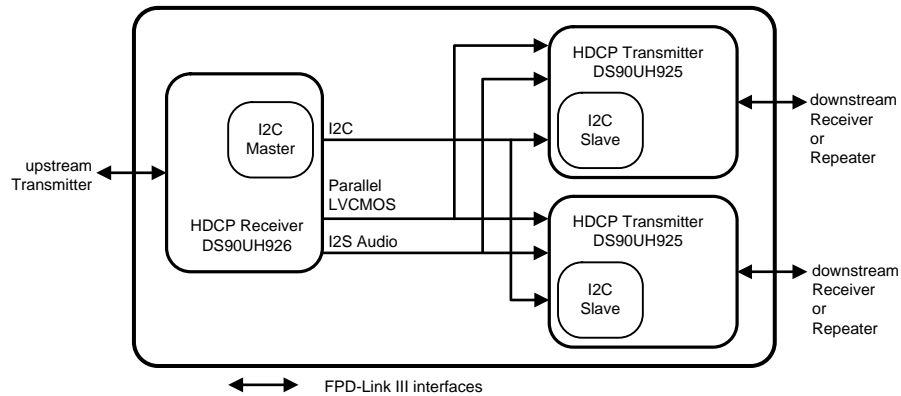
Figure 14. HDCP 1:2 Repeater Configuration
