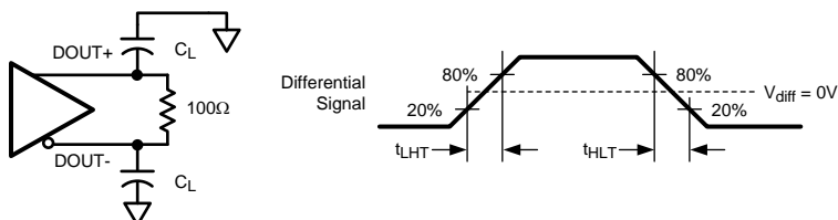
Figure 5. Serializer CML Output Load and Transition Time
