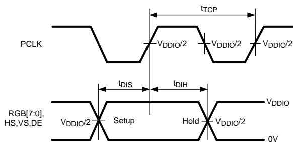
Figure 6. Serializer Setup and Hold Times
