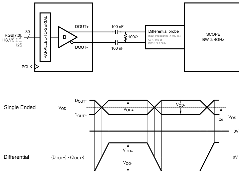
Figure 2. Serializer VOD DC Output
