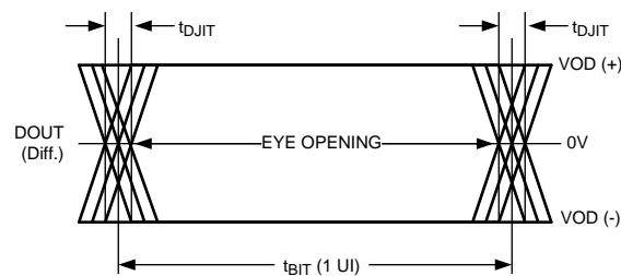
Figure 8. Serializer CML Output Jitter
