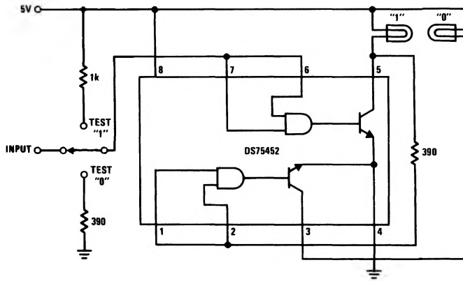
FIGURE 19. TTL or DTL Positive Logic-Level Detector
